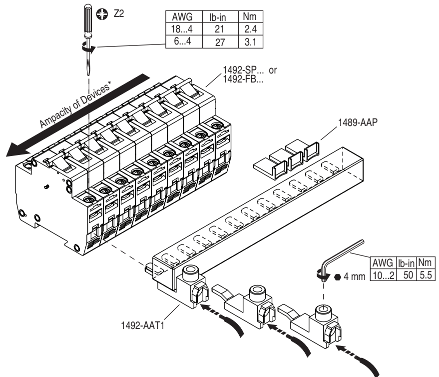
Figure 5 - Bus Bar Installation
